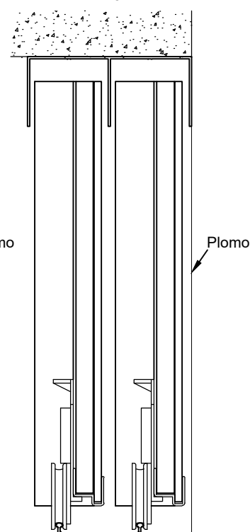
Detalle Vertical cantoneira de 15mm.
