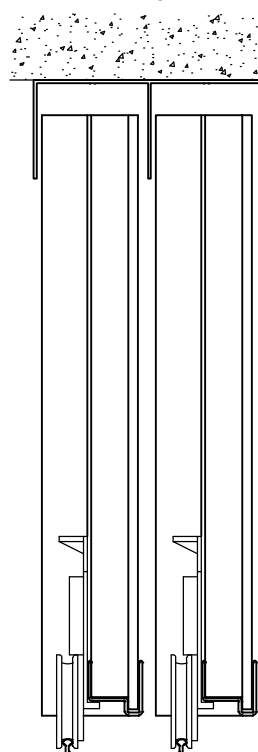
Detalle Vertical cantoneira de 18mm.
